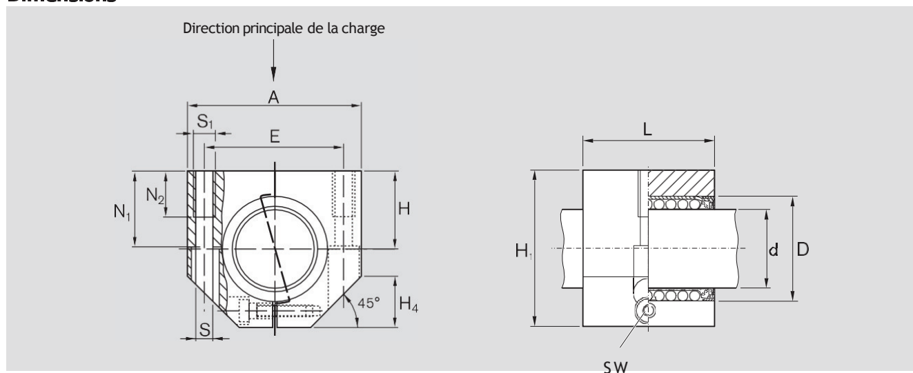
Dimensions (mm)
